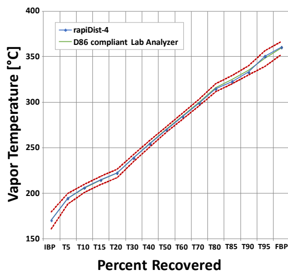
Fig. 2 Outstanding reproducibility and correlation of the rapiDist-4 with an ASTM D86 compliant laboratory analyzer. Repeatability limits according to ASTM D86 are marked as dotted lines.
